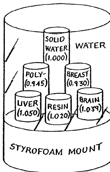
ELECTRON DENSITY PHANTOM (CONTRAST, CT LINEARITY)
