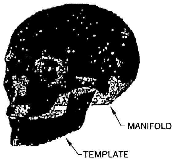
FITTED TEMPLATE SURFACE
